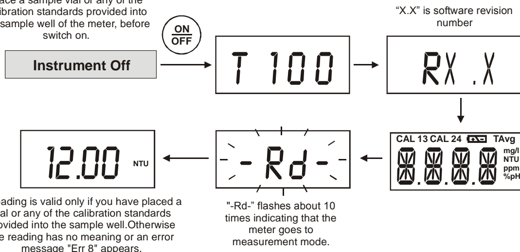
Figure 7: Power-up Sequence
